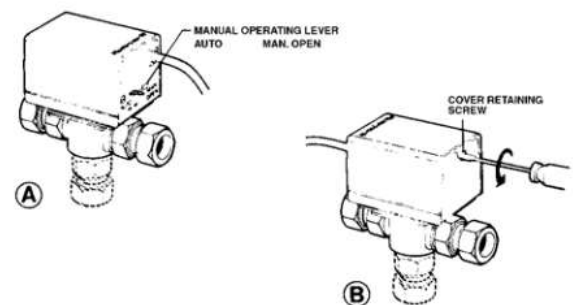
Fig. 1. Removing Cover
